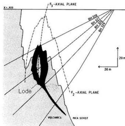
Schematic section across the Pirilä mineralisation. From Makkonen and Ekdahl (1988). Edited by P.Eilu (1999)
