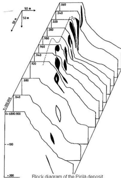
Block diagram of the Pirilä deposit. From Makkonen and Ekdahl (1988).
